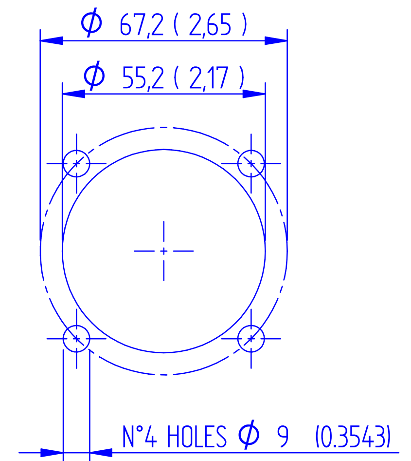
DRILLING JIG FOR JOINT D.48 - D.1.89
