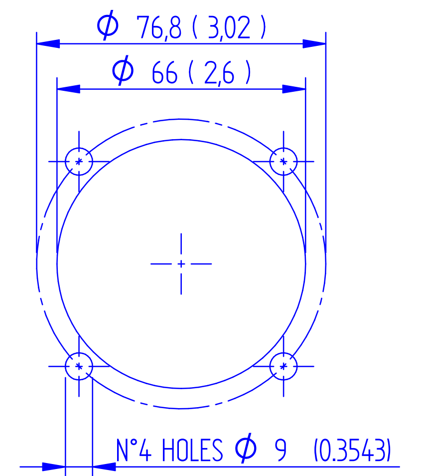
DRILLING JIG FOR JOINT D.60 - D.2.362
